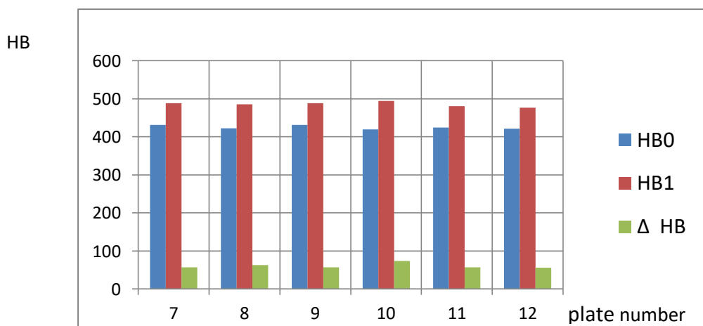
Figure 6.7 - The results of strengthening the non-grinding cutting inserts type WNMG 080408E-MC3 AP301M
