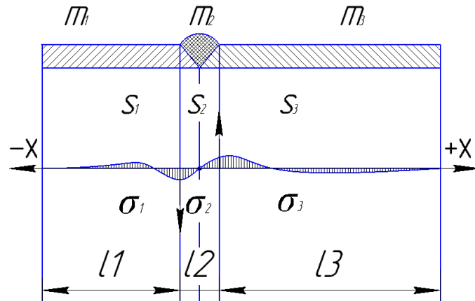
Figure 5.5 - Residual longitudinal stresses in the cross sections of the welded joint
