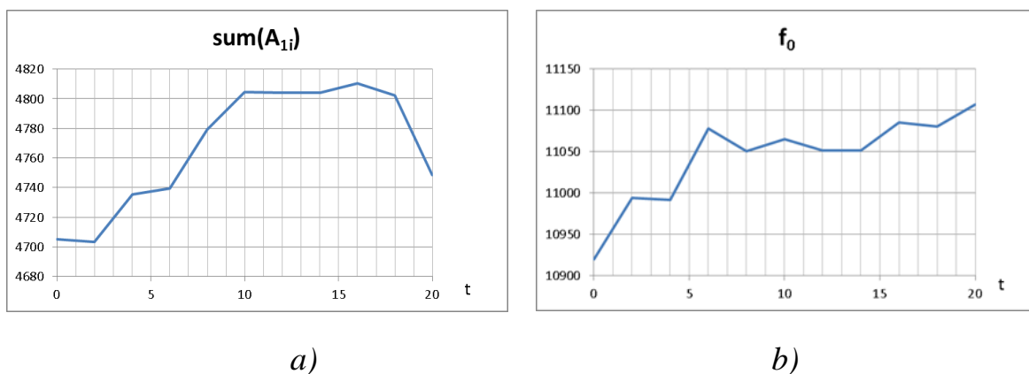
a - \sum_{i=1}^n A_i(f_{1i}); b - \text{resonant frequency } f_0 Figure 6.2 – Change in the performance and resonant frequency of the duralumin sample during resonant vibration treatment lasting 20 minutes with a discreteness of 2 minutes
