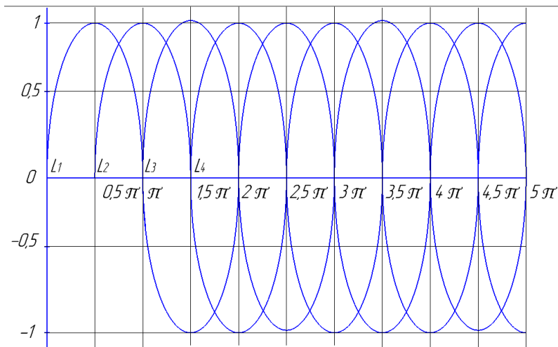
Figure 7.1 - Schematic diagram of a rotating magnetic field
